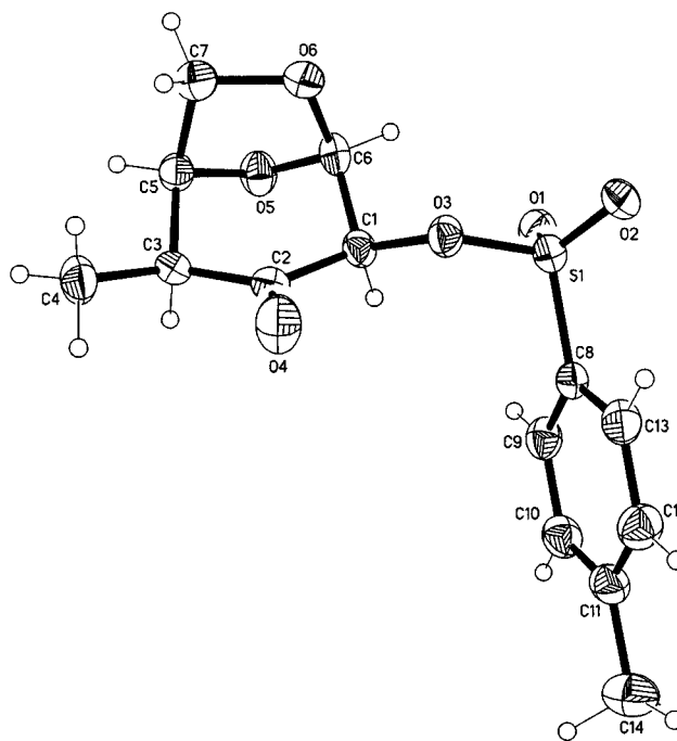
Figure 1. The molecular structure of 17 . Selected bond lengths [Å] and angles [°]: C1–O3 1.435(3), C2–O4 1.183(3), C6–O6 1.406(4), C7–O6 1.444(4), C1–C2 1.515(4), C1–C6 1.520(4), C2–C3 1.506(4), C3–C4 1.513(4), C3–C5 1.523(4), C5–C7 1.504(4); C5–O5–C6 102.3(2), C6–O6–C7 106.4(2).
