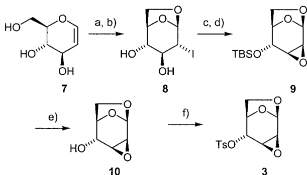
Scheme 2. a) (\text{Bu}_3\text{Sn})_2\text{O} , 3-Å molecular sieves, acetonitrile, reflux, 6 h; b) \text{I}_2 , room temp., 12 h, 68–79%; c) TBSCl, imidazole, DMF, room temp., 4 h; d) NaH (3 equiv.), 2 h, 85%; e) TBAF, THF, room temp., 20 min, 95%; f) TsCl, \text{Et}_3\text{N} , DMAP, \text{CH}_2\text{Cl}_2 , room temp., 2 h, 91%.
