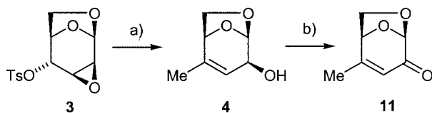
Scheme 3. a) \text{CuCN} (4 equiv.), \text{MeLi} (8 equiv.), \text{Et}_2\text{O}/\text{THF} , -78^\circ\text{C} (1 h) to -20^\circ\text{C} (2 h), 64%; b) PDC, \text{CH}_2\text{Cl}_2 , 18 h, 94%.
