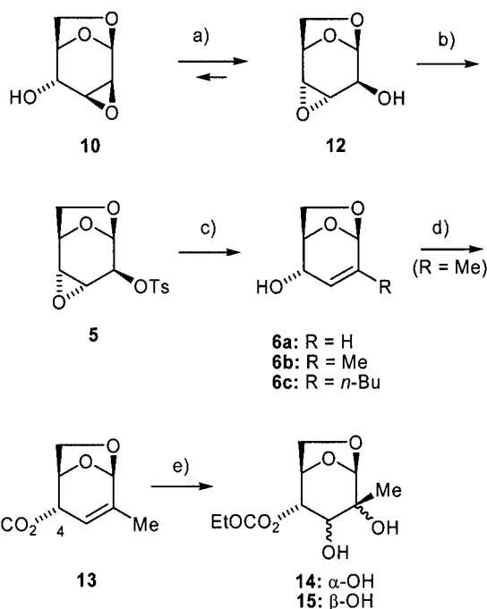
Scheme 4. a) NaOMe (4 equiv.), \text{CH}_2\text{Cl}_2 , (12 h), 95%; b) TsCl, \text{Et}_3\text{N} , DMAP, \text{CH}_2\text{Cl}_2 , 2 h, 92%; c) \text{CuCN} (4 equiv.), \text{RLi} (8 equiv.), \text{Et}_2\text{O}/\text{THF} , -78^\circ\text{C} (1 h) to -20^\circ\text{C} (2 h), 84%; d) TMEDA (0.6 equiv.), ethyl chlorocarbonate (1.2 equiv.), \text{CH}_2\text{Cl}_2 , (0.5 h), 90%; e) \text{OsO}_4 , NMO, acetone/ \text{H}_2\text{O} , 58%.
