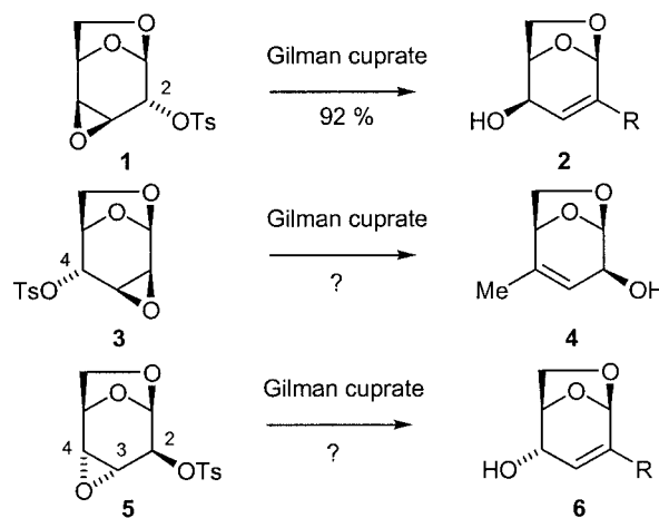
Scheme 1. Tandem epoxide→allyl alcohol rearrangement–cuprate cross-coupling of Černý epoxides 1 , 3 , and 5 with Gilman cuprates.
